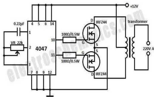
Fig7: Schematic of the DC to AC Inverter Circuit
