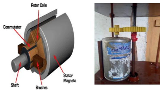
Fig4: Dynamo
